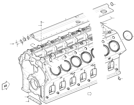
CRANKCASE XS595010.00024
