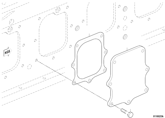
INSPECT PORT COVER XS593010.00008
