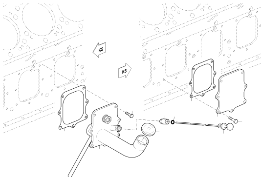
OIL FILLER NECK W. OIL DIPSTICK, LF XS595010.00056
